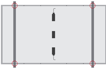
Bolt installation with outer quad holes (beam vertical to the long frame)
