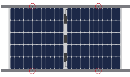
Bolt installation with inner quad holes (beam parallel to the long frame)
