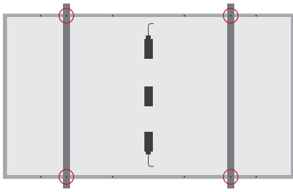
Bolt installation with inner quad holes (beam vertical to the long frame)
